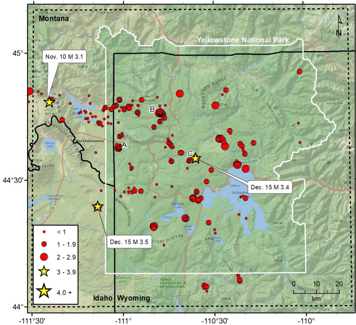
Figure 1. Epicenters of earthquakes located by the University of Utah Seismograph Stations, October 1, 2019, through December 31, 2019. Earthquake swarms (labeled A–C) are discussed in the text.
